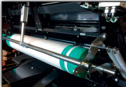
Patented front mounted PowerBind net system with low loading height and super-fast cycle time. Twin tube twine tie system also available.
