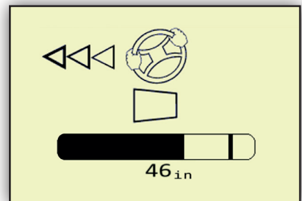
Three way driving indication showing bale shape and driving direction for perfect bale formation in all windrows.
